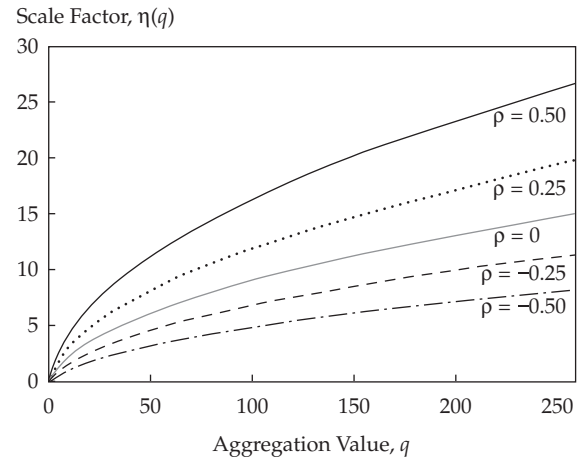
Figure 1. Scale Factors of Time-Aggregated Sharpe Ratios When Returns Follow an AR(1) Process: For \rho = -0.50, -0.25, 0, 0.25, and 0.50
